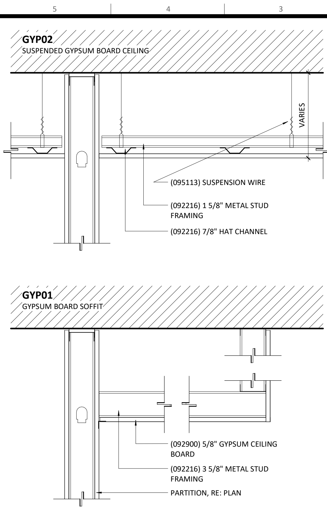
Ceiling Detail - Typical Ceiling Types K3 1 1/2" = 1'-0"
