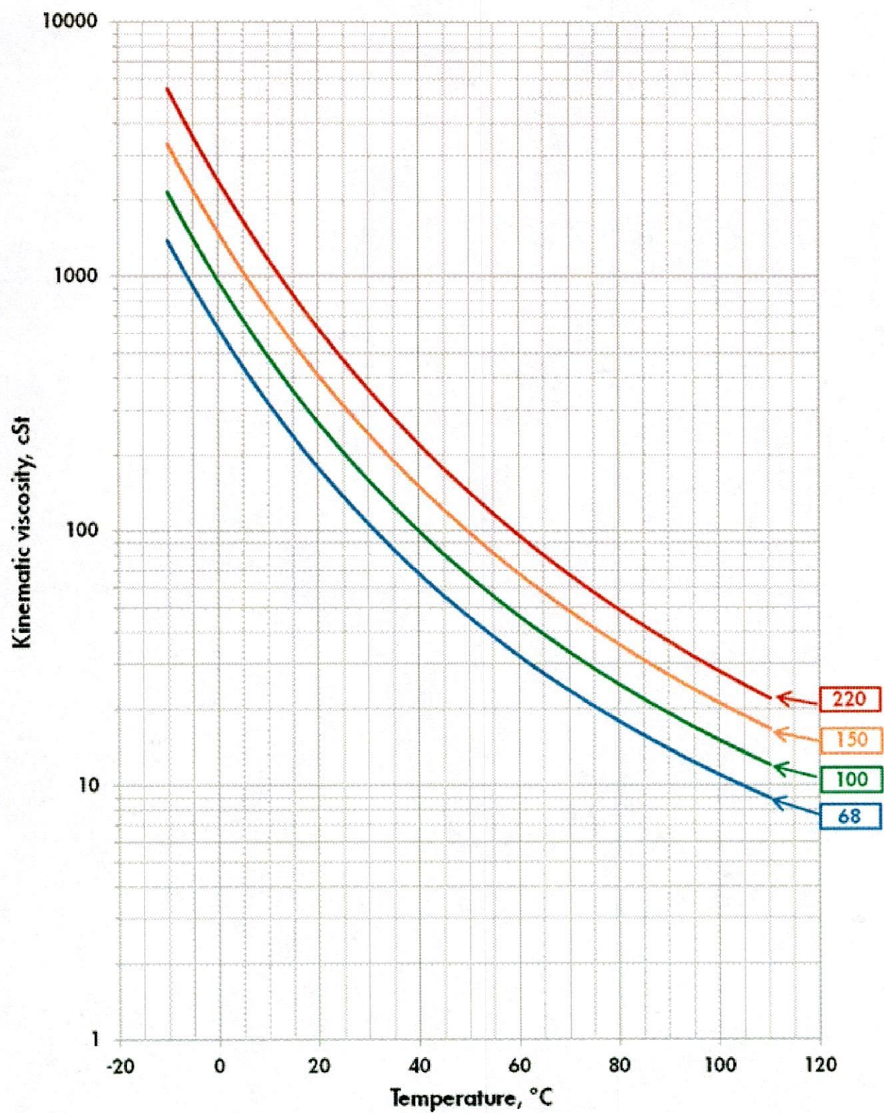
Viscosity - Temperature Diagram for Shell Morlina S4 B 68-220
