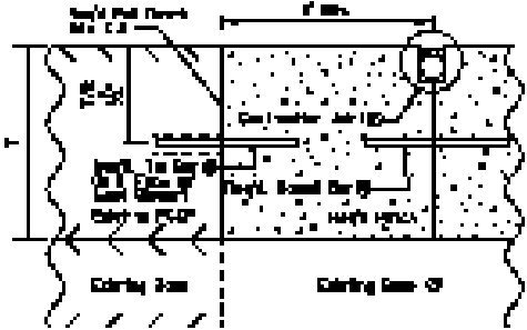
MATCHING DETAIL AT TRANSVERSE JOINT
